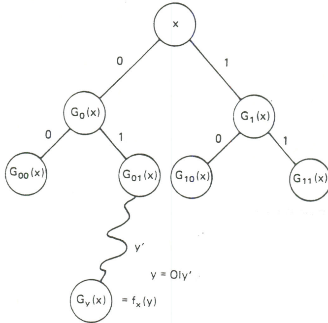
FIG. 1. The string f_x(y) is then stored in the leaf reachable from the root following the edge-path labeled y .
