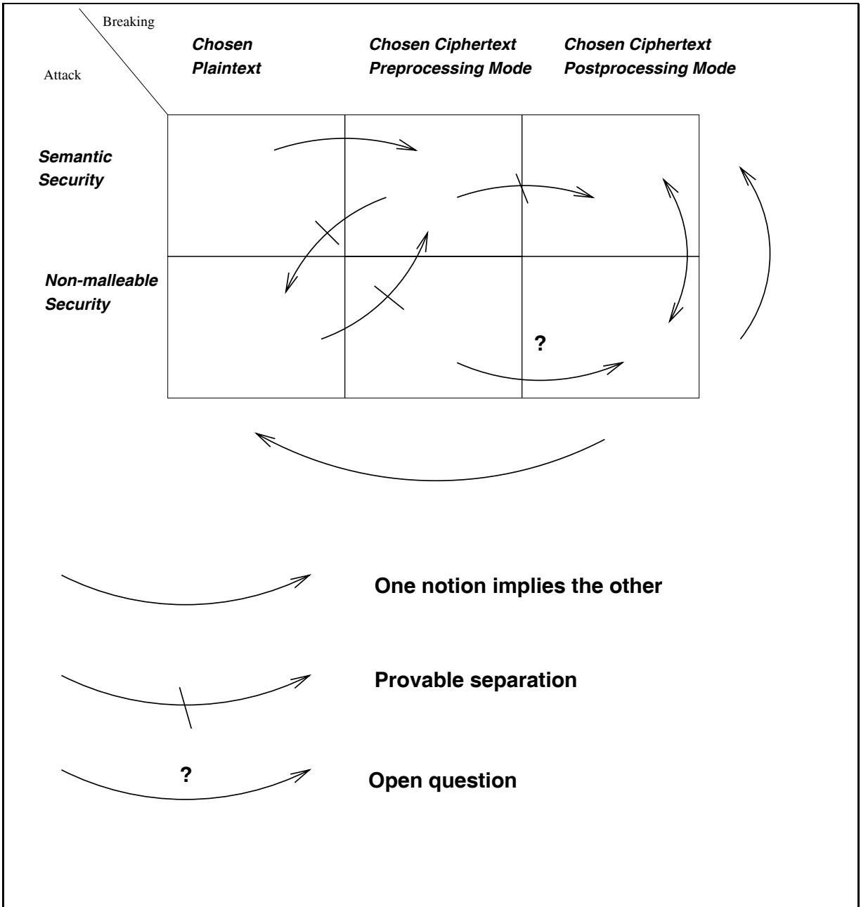
Figure 1: Relationship between security notions.
