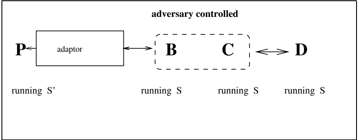
Figure 3: The S' -adaptor- S system used in constructing the Extractor
